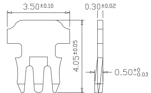
“1” : 3 PRONGS FOR SOLID WIRE(S) 單芯線用三叉型金片
