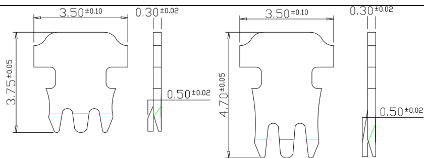
“3” : 3 PRONGS FOR STRANDED & SOLID WIRE(S) 多芯線及單芯線用三叉型金片
