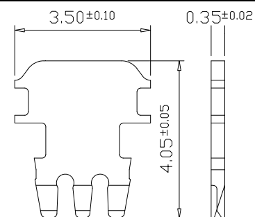
“ 5 ” : 3 PRONGS FOR SOLID WIRE(S) 單芯線用三叉型金片
