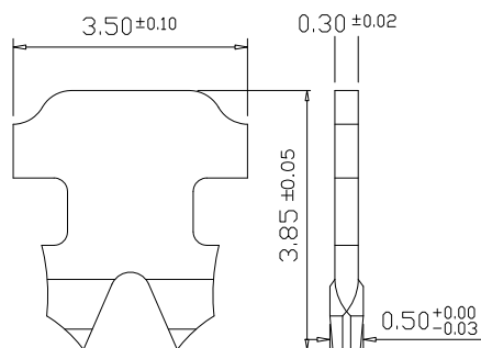
“ 2 ” : 2 PRONGS FOR SOLID WIRE(SS) 單芯線用大拐角型金片
