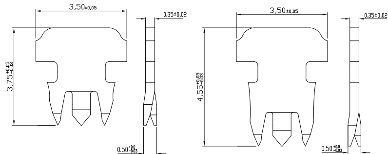
“G” : 3 PRONGS FOR STRANDED & SOLID WIRE(S) 多芯線及單芯線用三叉型金片
