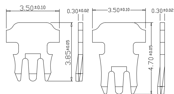
“ 3 ” : 3 PRONGS FOR SOLID WIRE(S) 單芯線用三叉型金片
