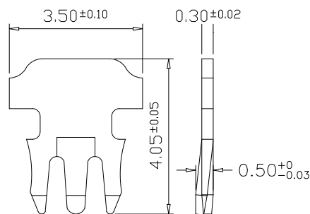
“3” : 3 PRONGS FOR STRANDED & SOLID WIRE(S) 多芯線及單芯線用三叉型金片
