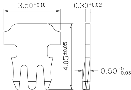
“3” : 3 PRONGS FOR STRANDED & SOLID WIRE(S) 多芯線及單芯線用三叉型金片
