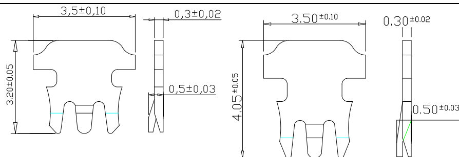
“3”：3 PRONGS FOR STRANDED & SOLID WIRE(S) 多芯線及單芯線用三叉型金片
